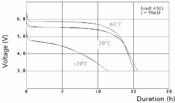
Temperature characteristics
