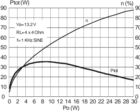
Figure 14. Power dissipation & efficiency vs. output power (sine-wave operation)
